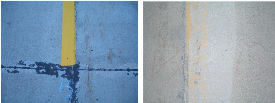
Figure 6.10. Concrete pavement condition before (left) and after (right) paint has been removed by grinding
