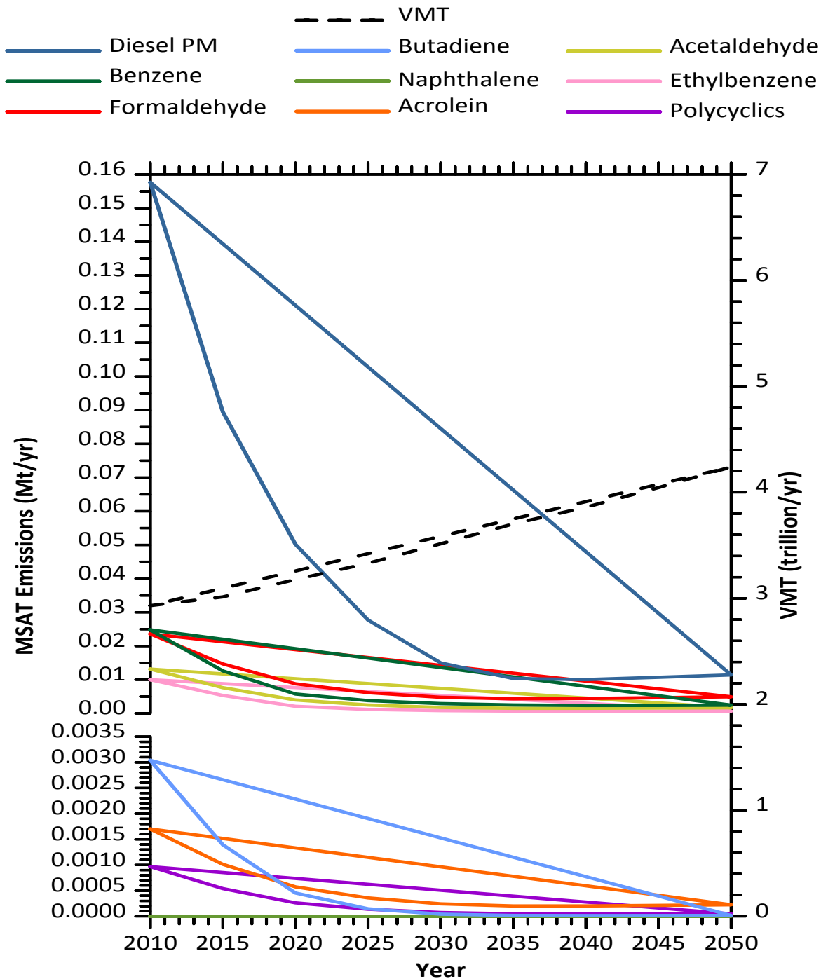
Figure 1: FHWA PROJECTED NATIONAL MSAT EMISSION TRENDS 2010 – 2050 FOR VEHICLES OPERATING ON ROADWAYS USING EPA’S MOVES2014a MODEL
