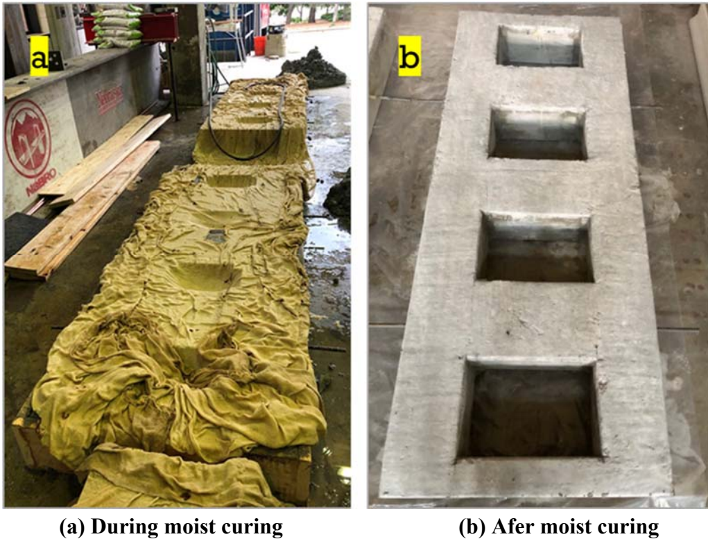
Figure 5-4. Slab curing.
