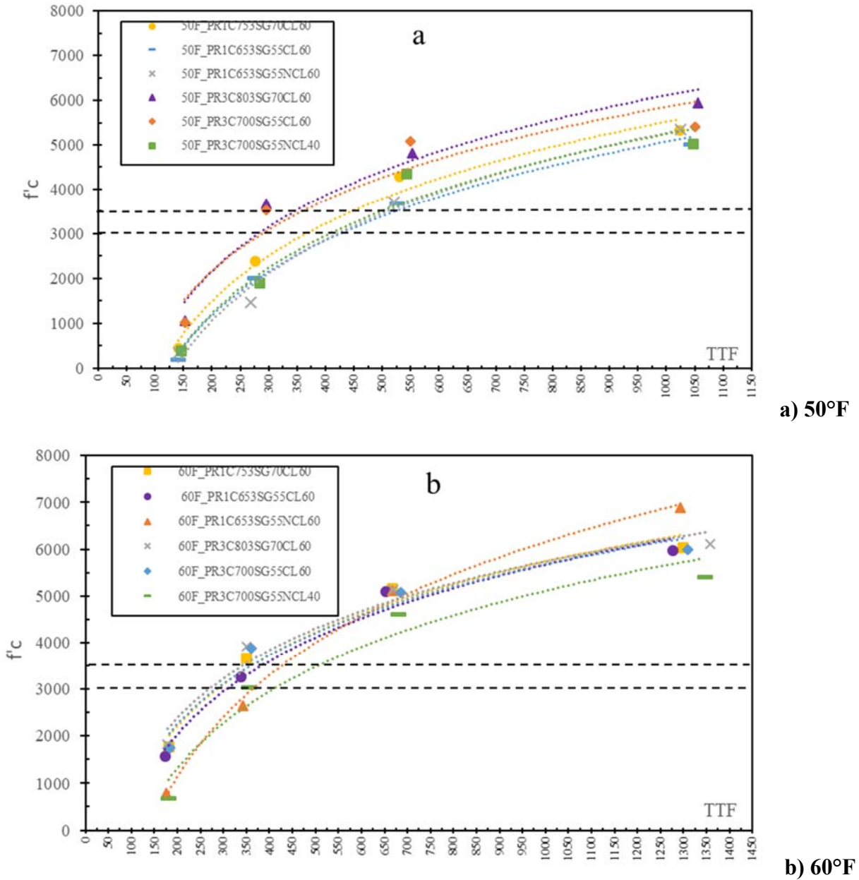
Figure 4-14. Maturity analysis at different ages for ambient temperatures.
