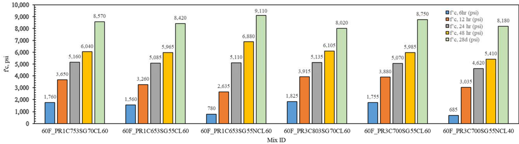
Figure 4-13. Compressive strength of Phase 3 mixes cured at 60°F.
