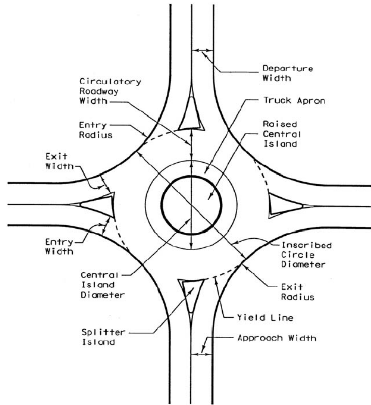
Figure 1 - Key roundabout features (source: 8)
