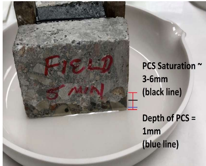
Figure 4 - Blocks were soaked in PCS at a depth of 1mm. The PCS wicked up the block 3-6 mm.
