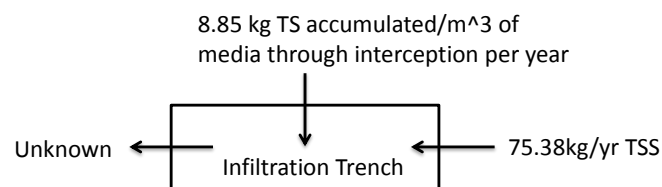
Figure 4.2 Yearly mass balance for TS accumulation in the infiltration trench
