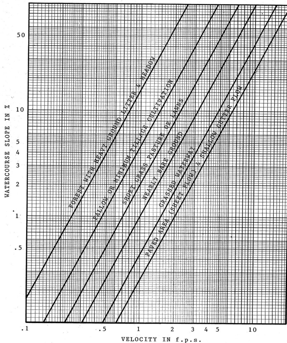
Figure 2.3 Velocities for estimating travel time (Olsson Associates 2006)
