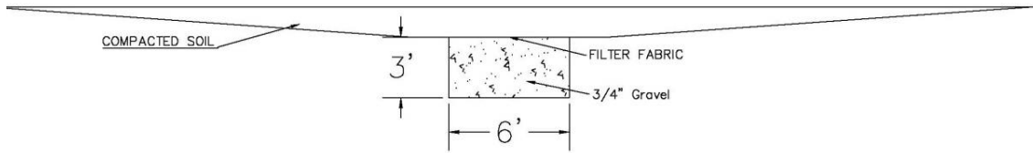
Figure 2.13 Check dam filter cross section
