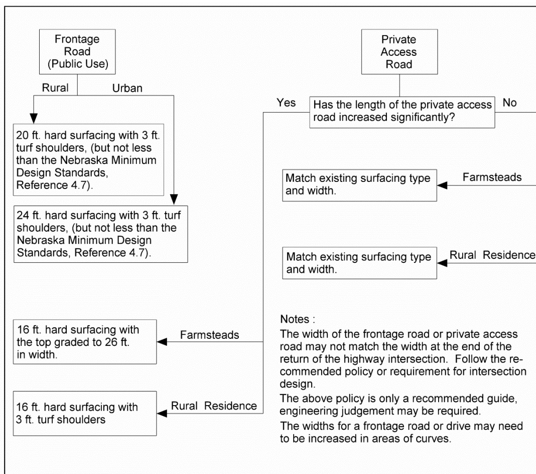
Exhibit 4.4 Flow Chart for Roadway Widths of Frontage Roads and Access Roads
