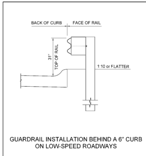
Exhibit 9.26 9.25 Guardrail Installed Behind a Six-Inch Curb on a Low-Speed ( \leq 45 mph) Roadway
