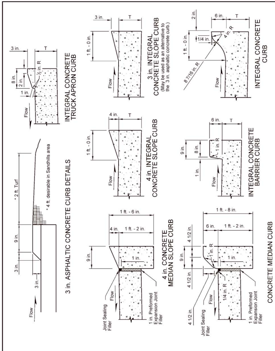
Exhibit 6.12 Typical Curb Details
