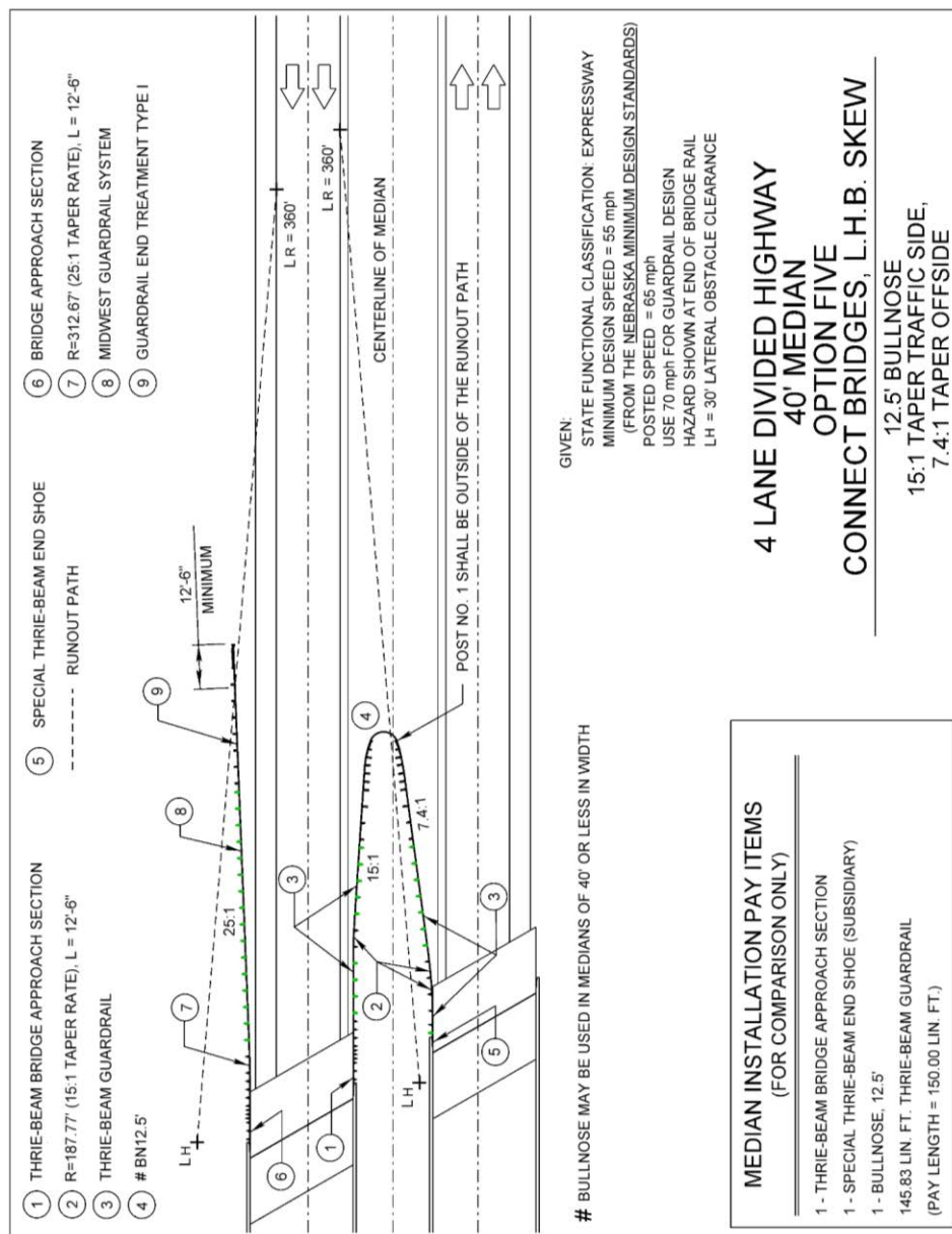
Exhibit 9.24 9.23 Example Bullnose Bridge Connection in a 40 Foot Wide Median: Left-Hand-Back Skew, Tapered Bullnose, Bridges Connected
