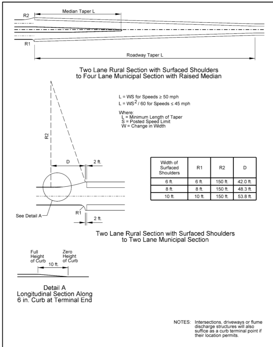
Exhibit 6.14 Examples of Rural to Urban Roadway Transitions
