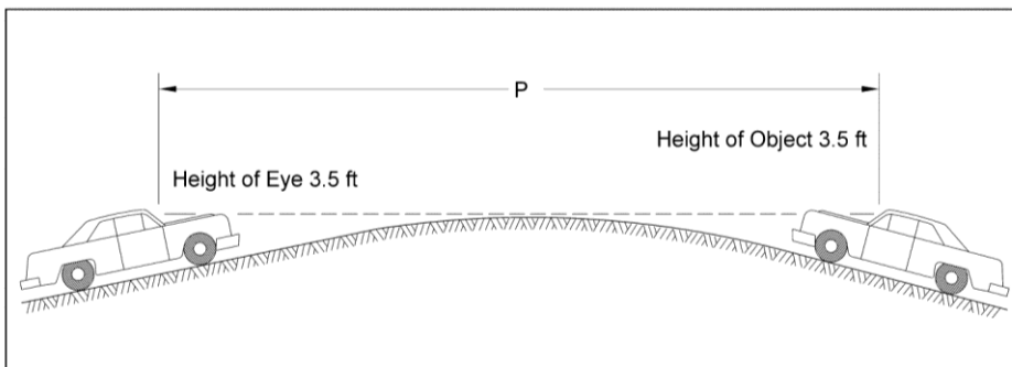
Exhibit 3.12 Passing Sight Distance Design Considerations
