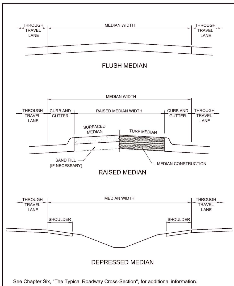
Exhibit 4.23 Median Types
