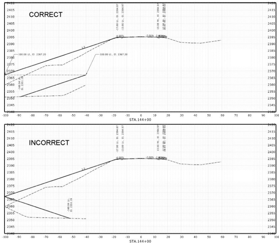
Exhibit 11.4 Roadway Cross-Section Break Lines
