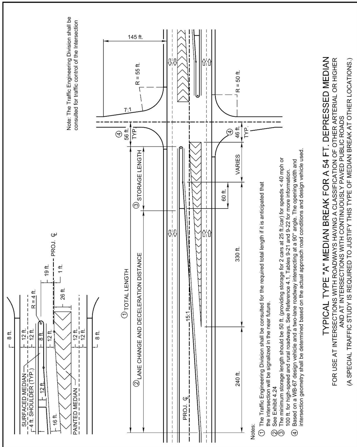
Exhibit 4.36 Typical Type A Median Break (54 Foot Depressed Median)
