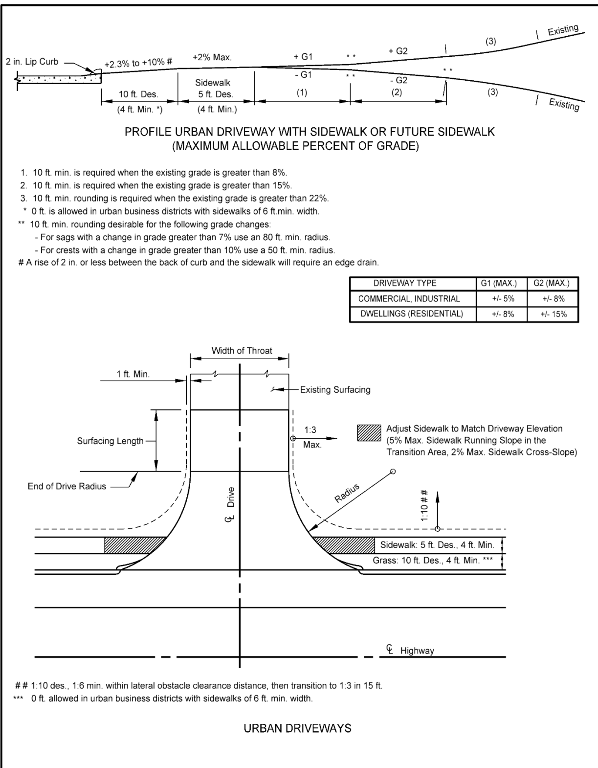
Exhibit 4.18 Urban Driveway
