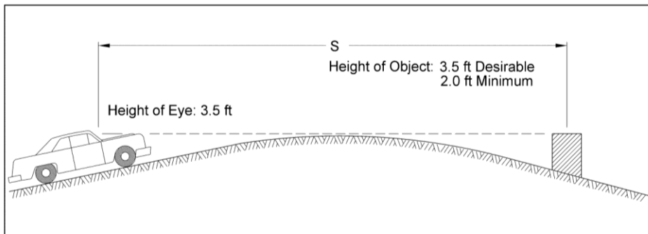
Exhibit 3.11 Crest Vertical Curve Design Elements
