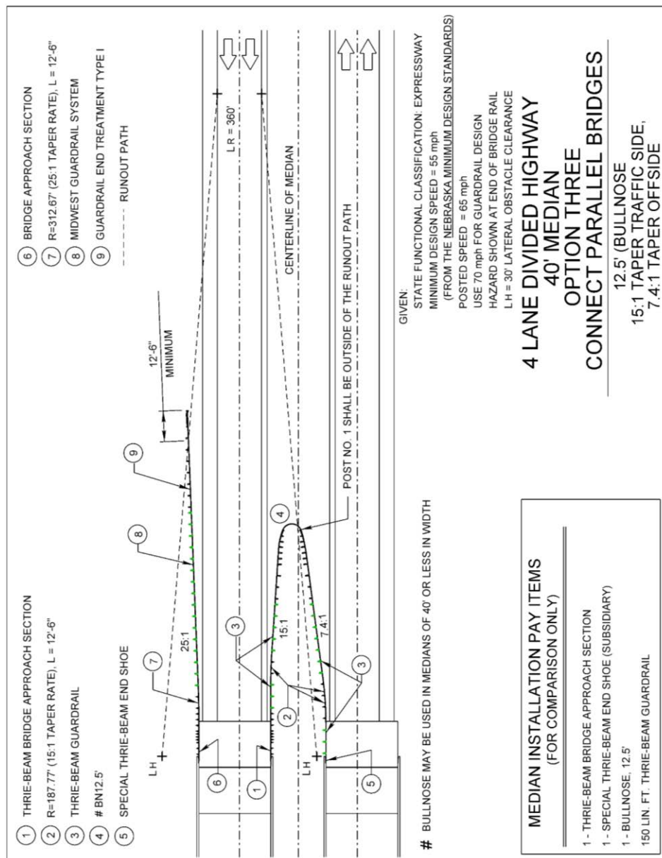
Exhibit 9.22 9.21 Example Bullnose Bridge Connection in a 40 Foot Wide Median: Tapered Bullnose, Bridges Connected
