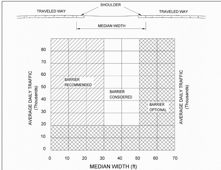
Exhibit 9-15 9.14 Guidelines for Median Barriers Source: Roadside Design Guide (Ref. 9.1)
