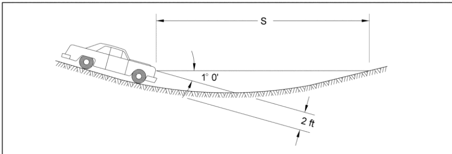
Exhibit 3.13 Sag Vertical Curve Design Elements
