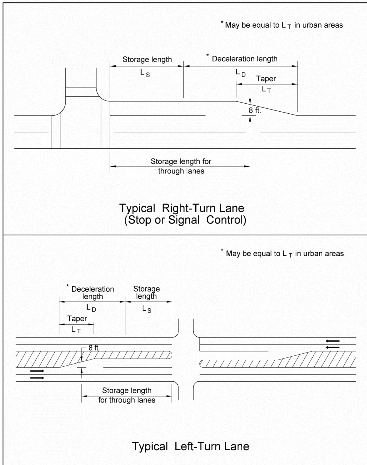
Exhibit 4.10 Typical Auxiliary Lanes
