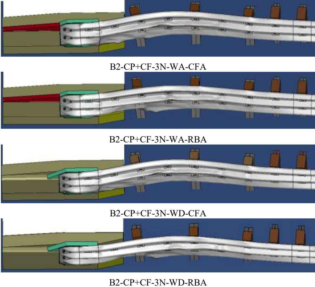
Figure 90. System Damage, Buttrass 2
