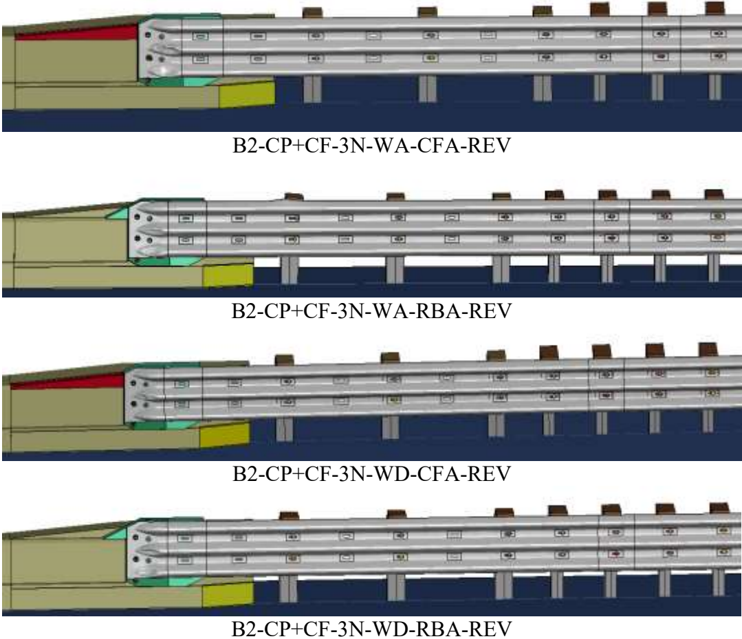
Figure 95. System Damage for Reverse-Direction Impacts, Buttriss 2
