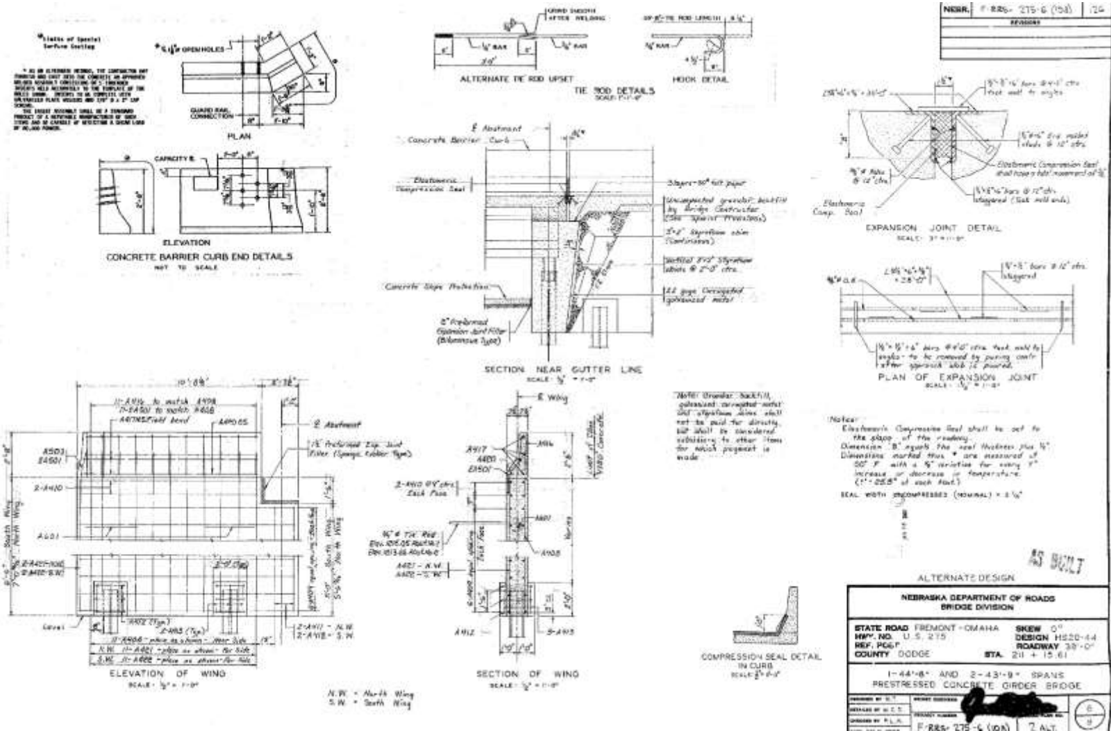
Figure A-9. NDOT Design Details, Buttruss 9
