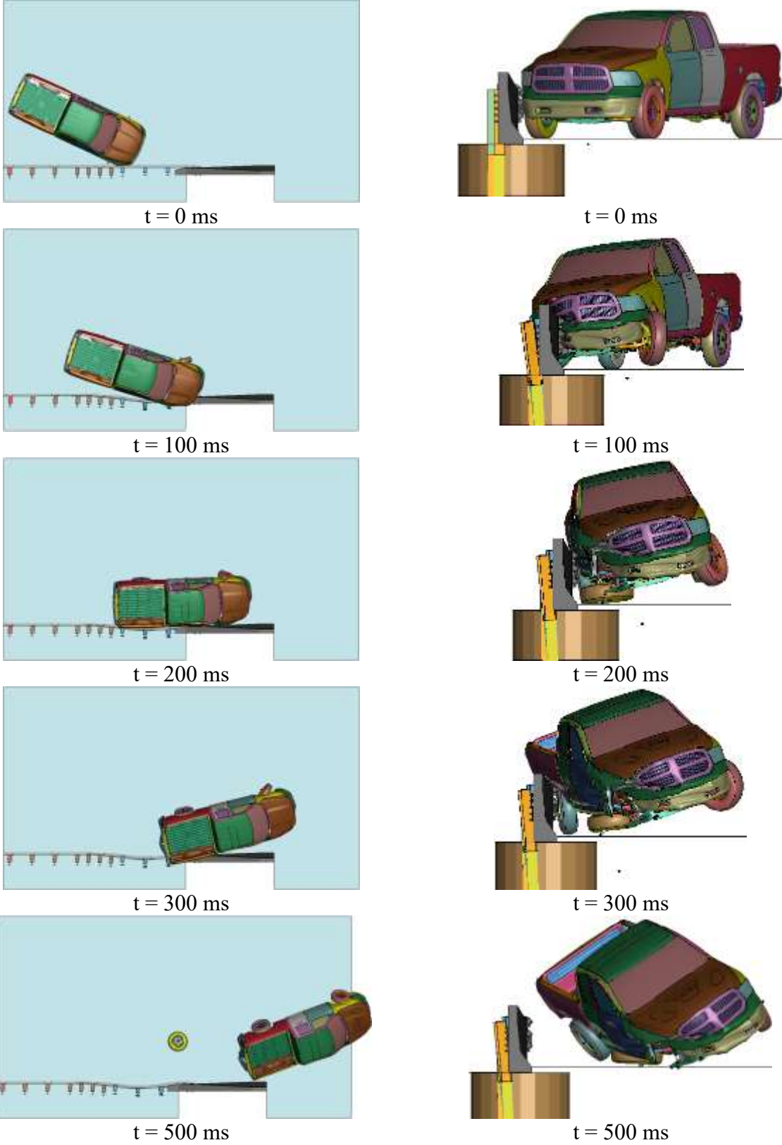
Figure 69. Sequential Images, Simulation No. B8-CP+CF-3N-WD
