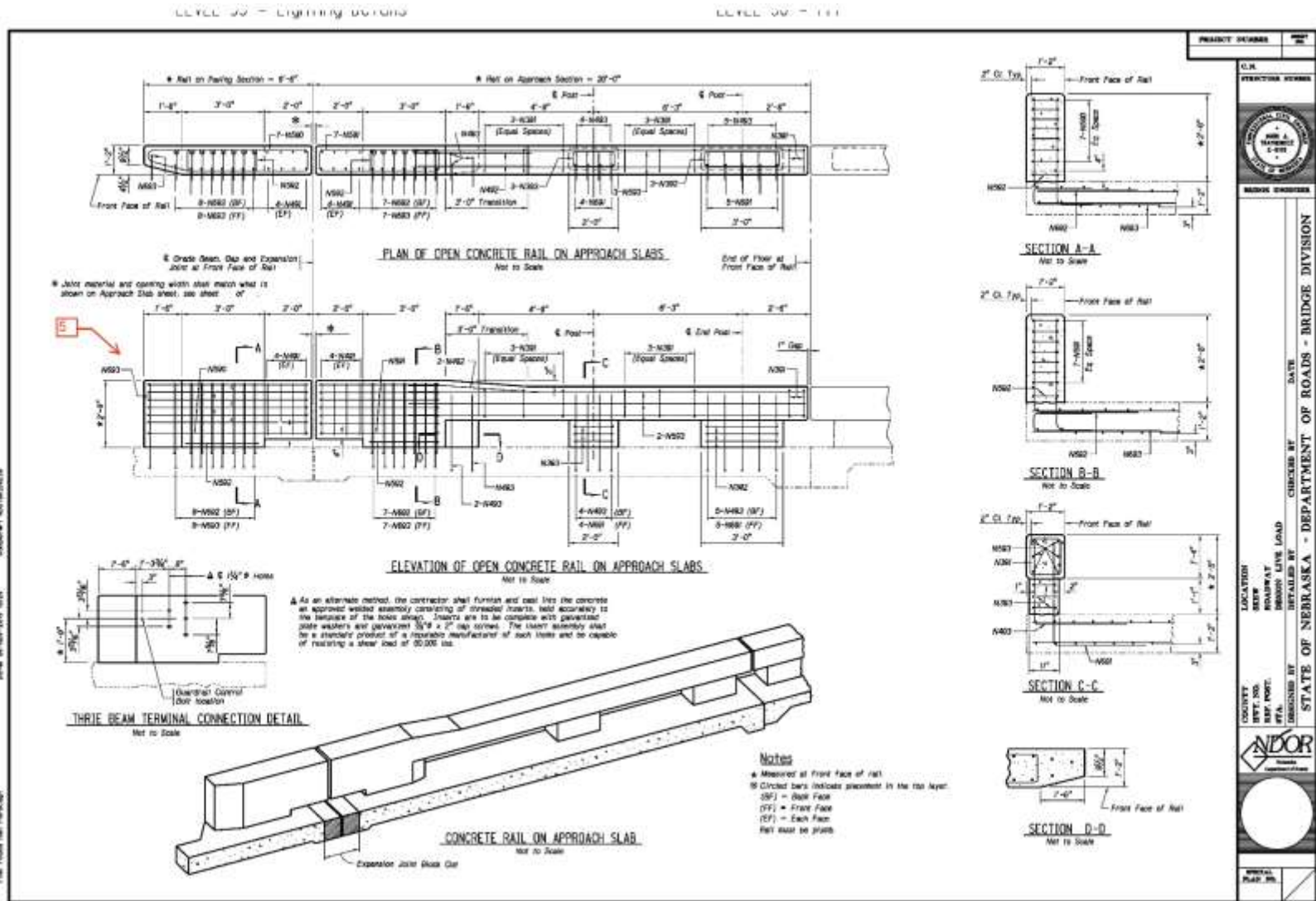
Figure A-5. NDOT Design Details, Buttrass 5
