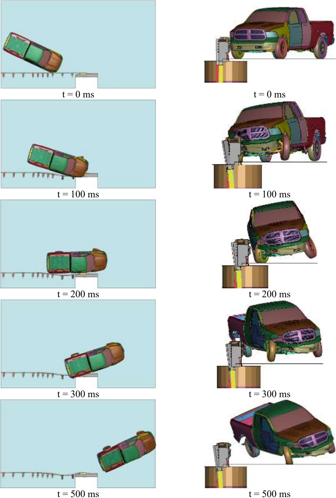
Figure 88. Sequential Images, Simulation No. B2-CP+CF-3N-WA-RBA
