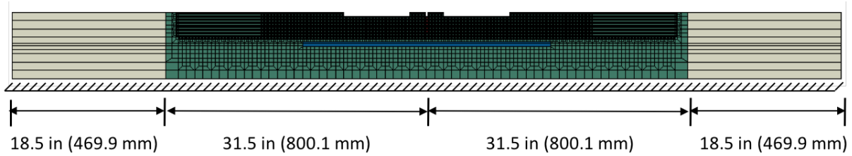
(a) A schematic cross-sectional profile of a concrete pavement structure and its mesh
