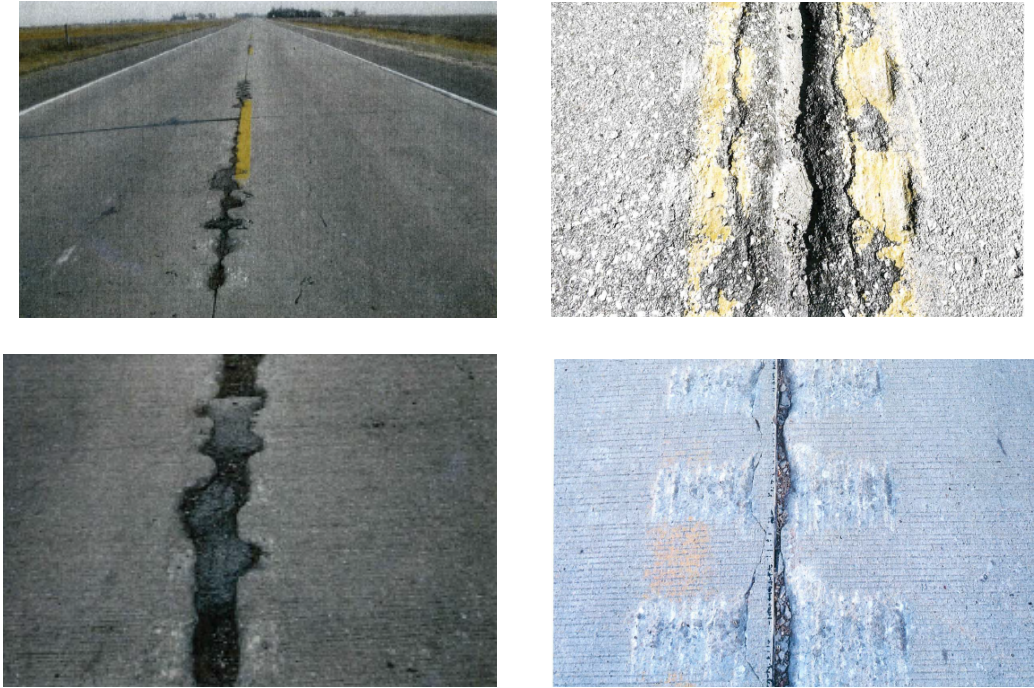
Figure 1-3. Pavement damage associated with CLRSs.
