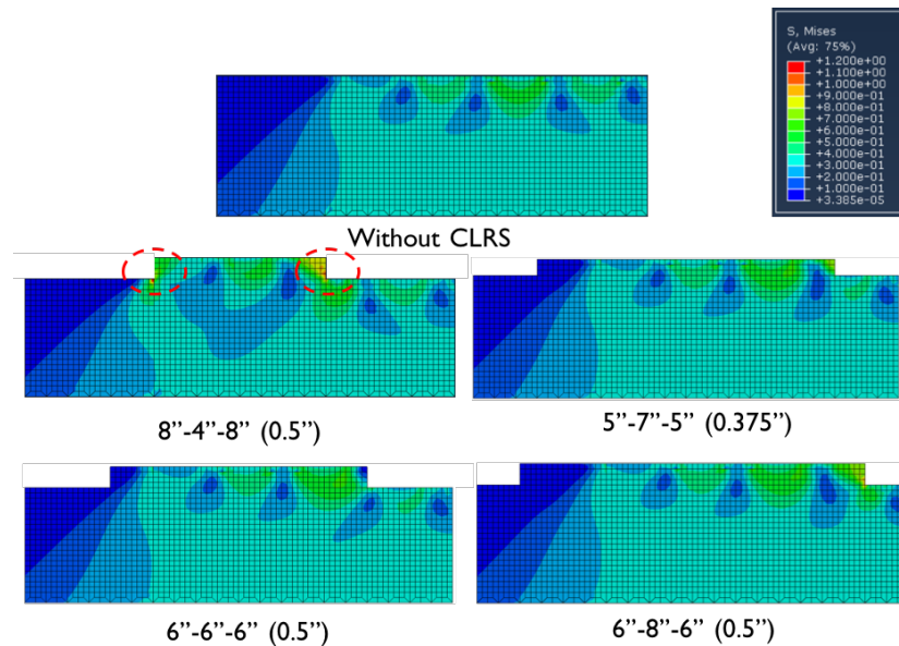
Figure 4-7. Stress contour plots of composite pavement without and with CLRSs: 2 nd loading.
