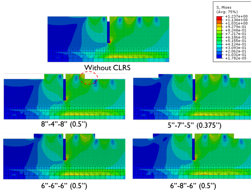
Figure 4-14. Stress contour plots of concrete pavement without and with CLRSs: 2 nd loading.
