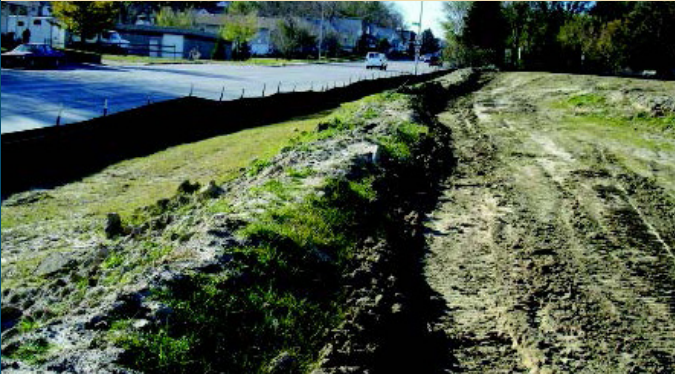
Pictured: Good example of a soil berm used for perimeter control.
