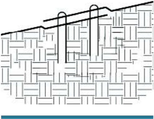
Figure: Place blankets parallel with the direction of flow. A minimum overlap of 8 inches is used to splice rolls together.
